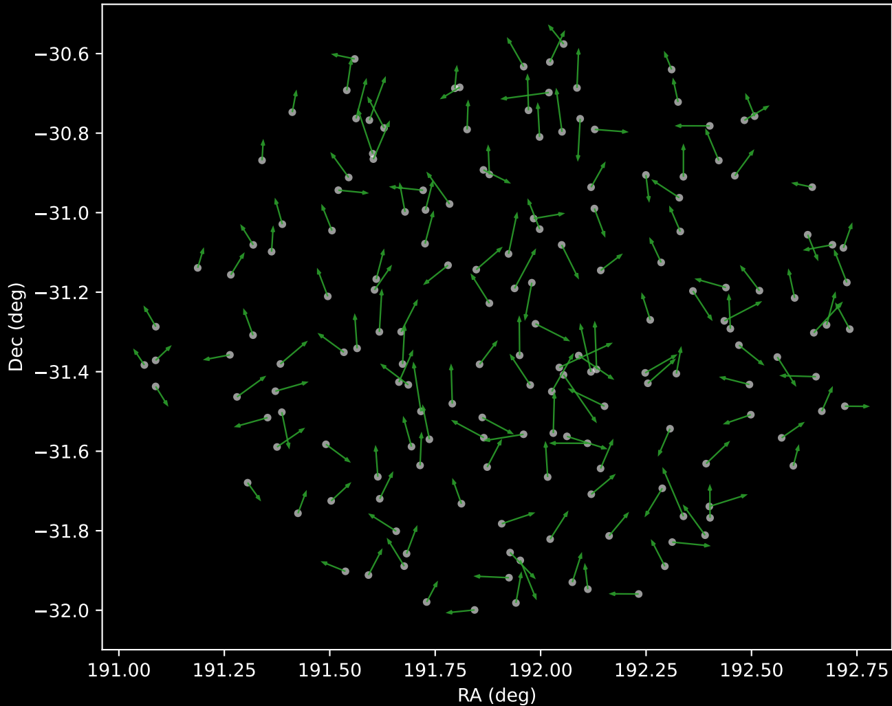
GALAH DR4 Cluster 4 Proper Motion Vectors (n=169)
