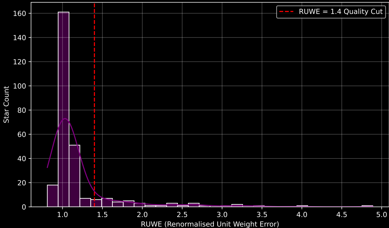
GALAH DR4 Field [1779] RUWE Distribution (n= 278)
