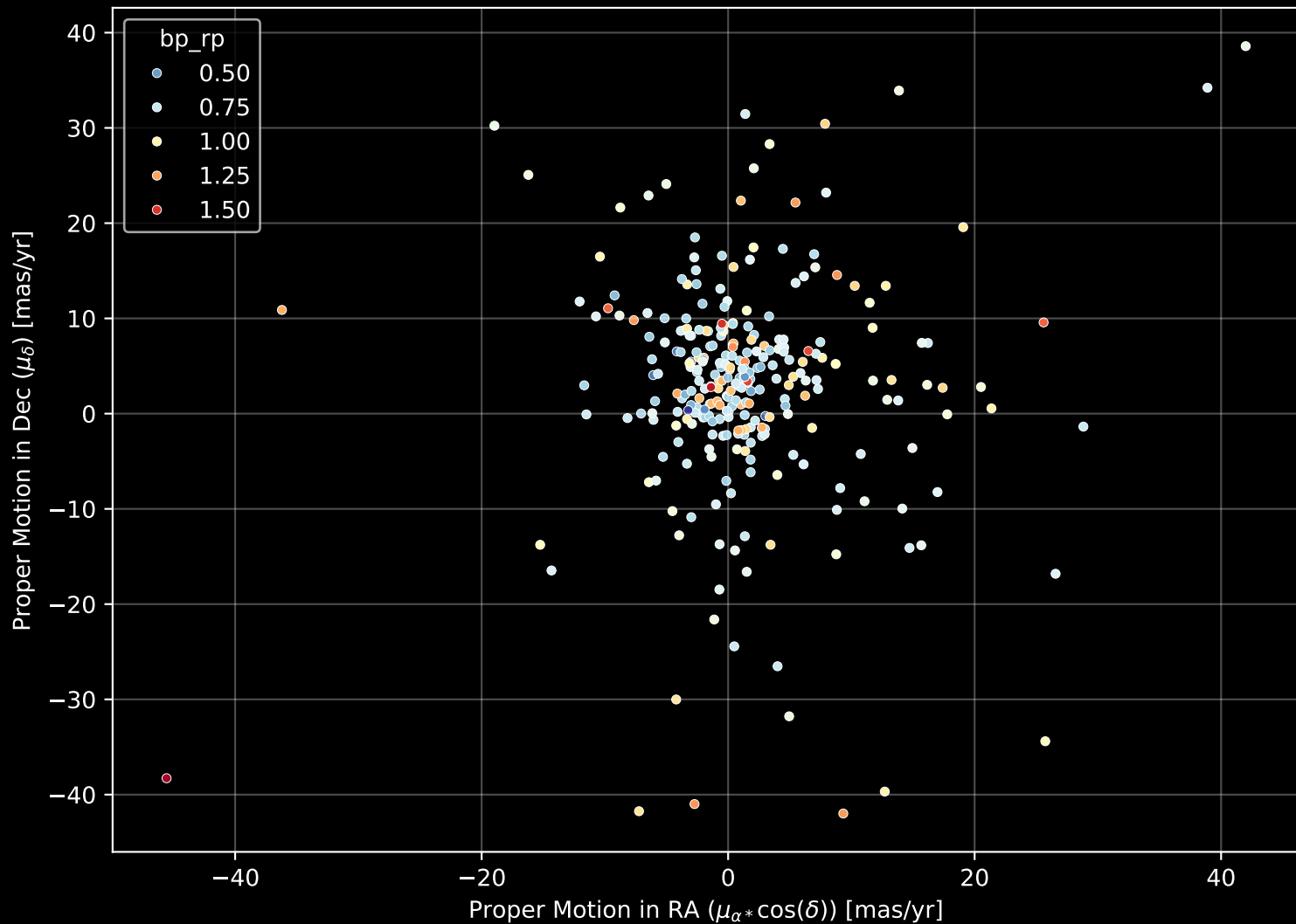
GALAH DR4 Field: [1779] Proper Motion Diagram (n= 285)
