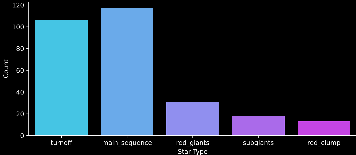
GALAH DR4 Field: [1779] Count plot of Star Type
